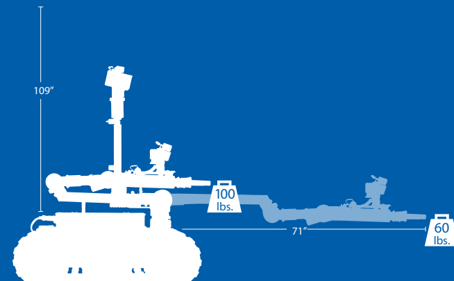
Vertical / Horizontal Extension and Weight Capacities
